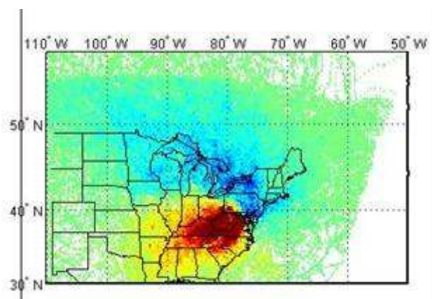
Sulfate
