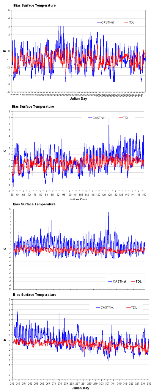
Figure 2-5. 2002 Seasonal Hourly Average Bias of Temperature
