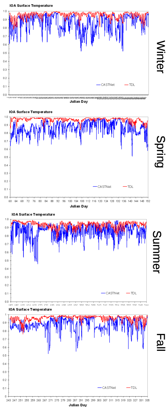
Figure 2-6. 2002 Seasonal Hourly Average Index of Agreement
