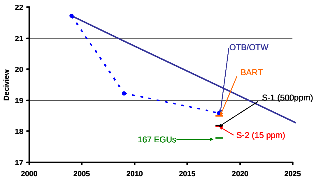
Figure 5-14. Visibility improvement relative to uniform rate of progress at Roosevelt-Campobello International Park
