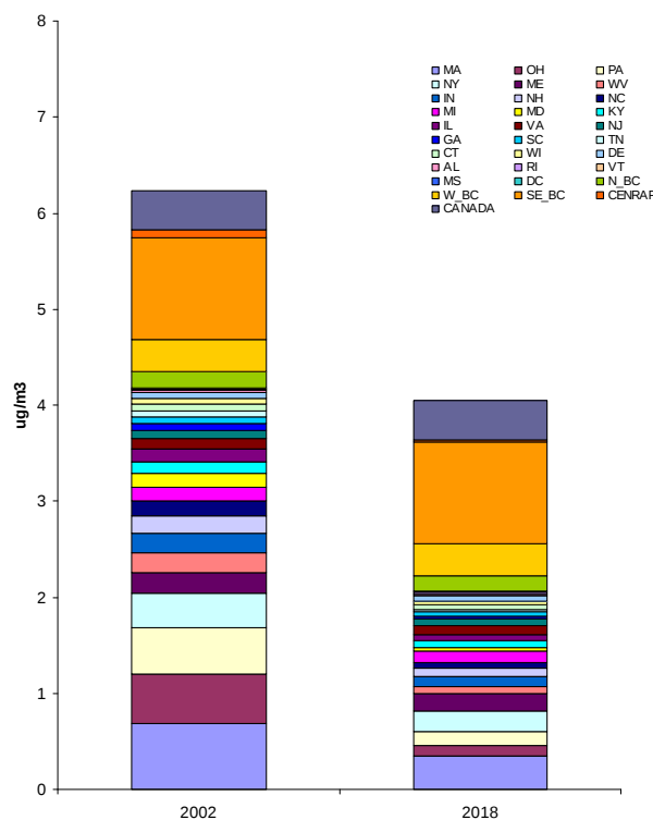
b. 2002 and 2018 sulfate mass from at Acadia National Park, twenty percent worst days apporportioned by REMSAD
