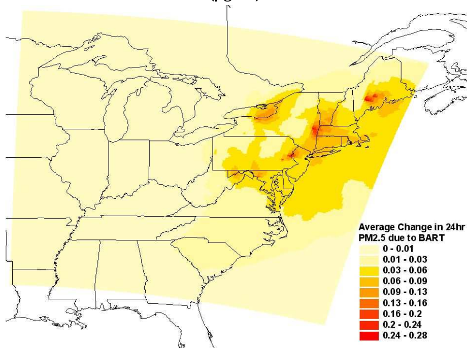
Figure 5-4. Average change in 24-hr PM 2.5 due to BART emission reductions ( \mu\text{g}/\text{m}^3 )
