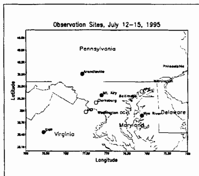
Figure 1. Map of the B-W region showing surface air quality sites and locations of aircraft profiles (solid circles) and upper air meteorological sounding sites (open circles) referred to in this paper.
