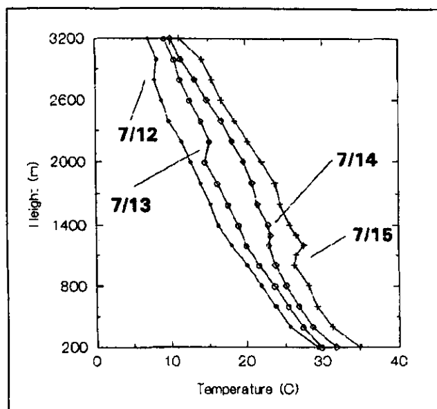
Figure 3. Temperature soundings for the lower troposphere at approximately 1800 UTC on July 12–15, 1995 near Clarksburg, MD.
