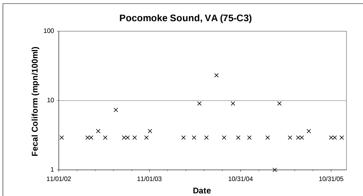
Figure 2.2.10: Observed Fecal Coliform Concentrations at Station 75-C3
