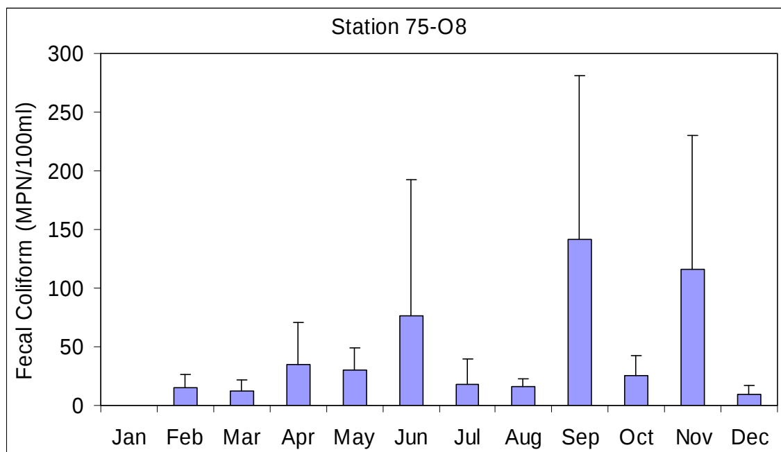
Figure C-7: Seasonality analysis of fecal coliform at Pocomoke River Station 75-O8 (VA)
