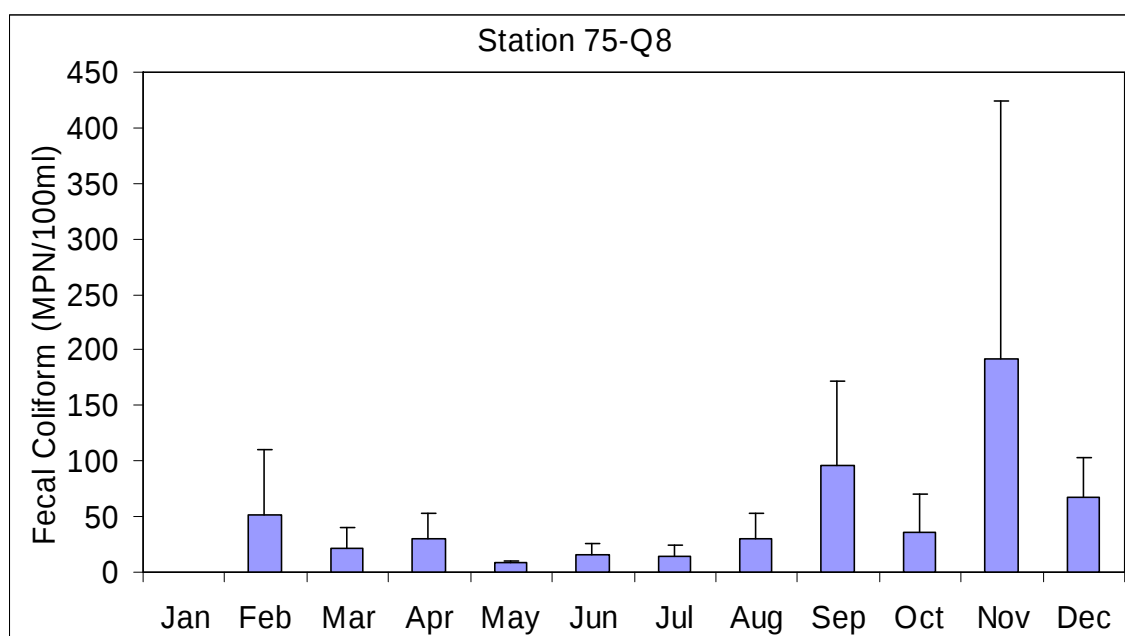
Figure C-9: Seasonality analysis of fecal coliform at Pocomoke River Station 75-Q8 (VA)
