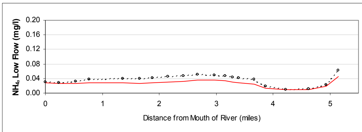
Figure A47: Ammonia vs. River Mile for the Future Low Flow TMDL Scenario
