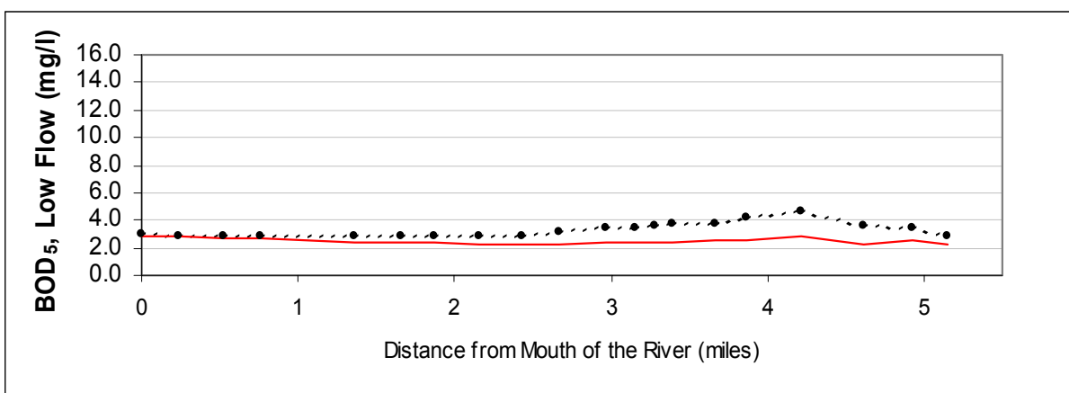
Figure A50: BOD vs. River Mile for the Future Average Flow TMDL Scenario
