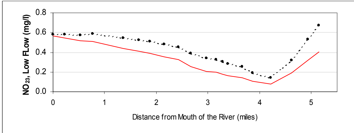
Figure A53: Nitrate (plus Nitrite) vs. River Mile for the Future Average flow TMDL Scenario
