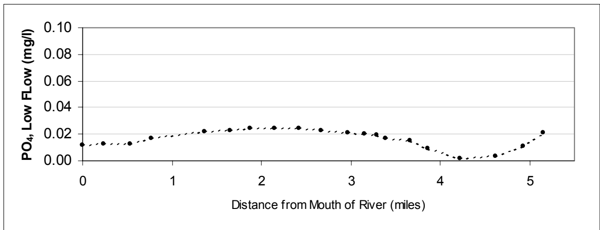
Figure A41: Ortho-Phosphorus vs. River Mile for the Baseline Conditions Average Flow Scenario
