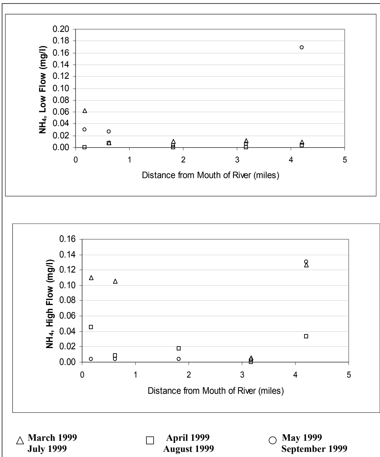
Figure A5: Longitudinal Profile of Ammonia Data
