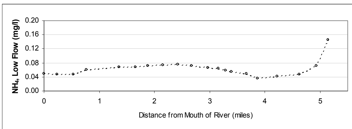
Figure A39: Ammonia vs. River Mile for the Baseline Conditions Average Flow Scenario
