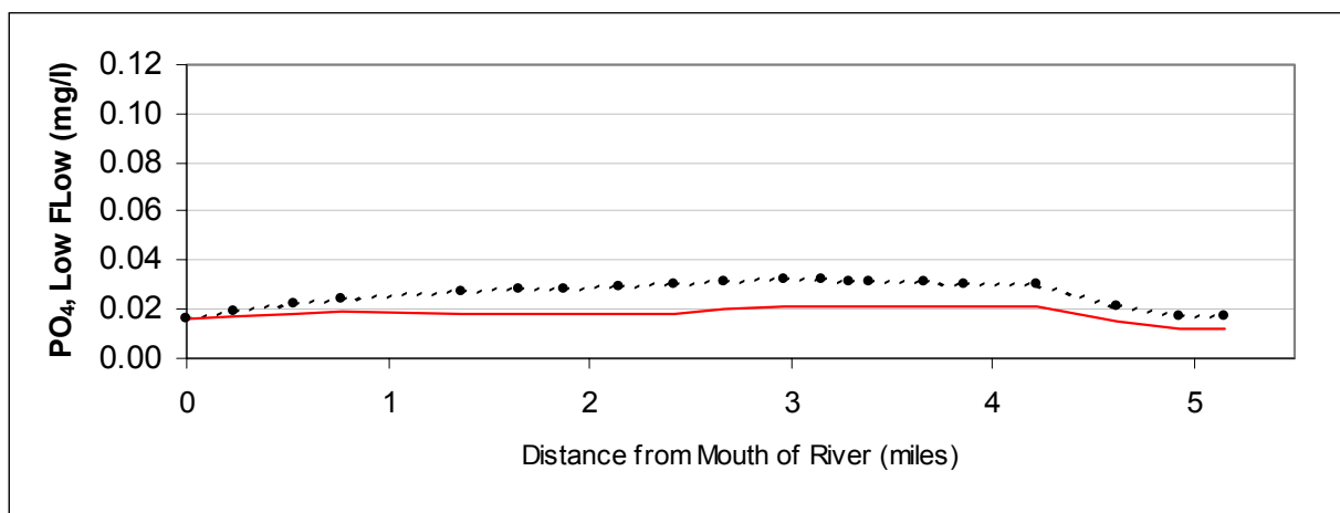
Figure A49: Ortho-Phosphate vs. River Mile for the Future Low Flow TMDL Scenario
