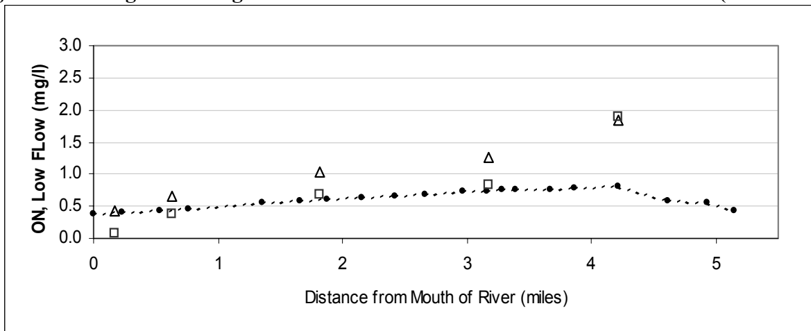
Figure A14: Organic Nitrogen vs. River Mile for the Calibration of the Model (Low flow)
