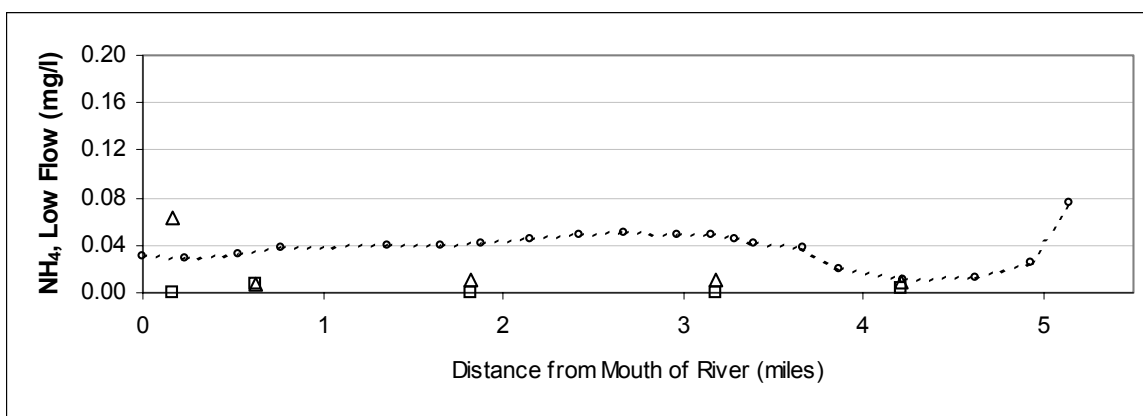
Figure A15: Ammonia vs. River Mile for the Calibration of the Model (Low flow)
