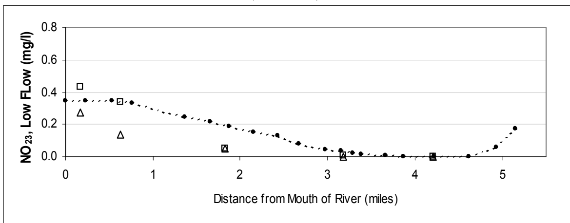
Figure A13: Nitrate (plus Nitrite) vs. River Mile for the Calibration of the Model (Low flow)
