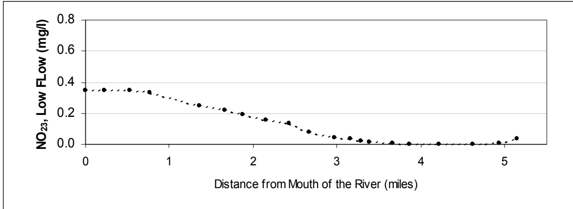
Figure A30: Organic Nitrogen vs. River Mile for the Baseline Conditions Low Flow Scenario
