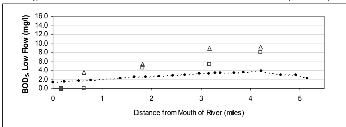
Figure A10: BOD vs. River Mile for the Calibration of the Model (Low flow)
