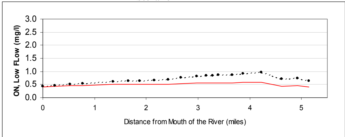
Figure A54: Organic Nitrogen vs. River Mile for the Future Average Flow TMDL Scenario
