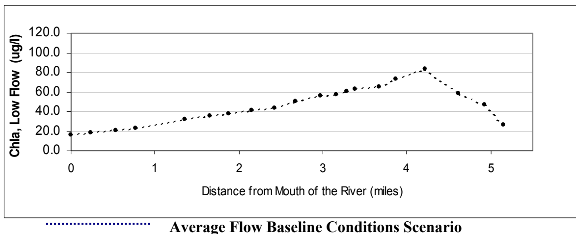
Figure A36: Chlorophyll a vs. River Mile for the Baseline Conditions Average Flow Scenario
