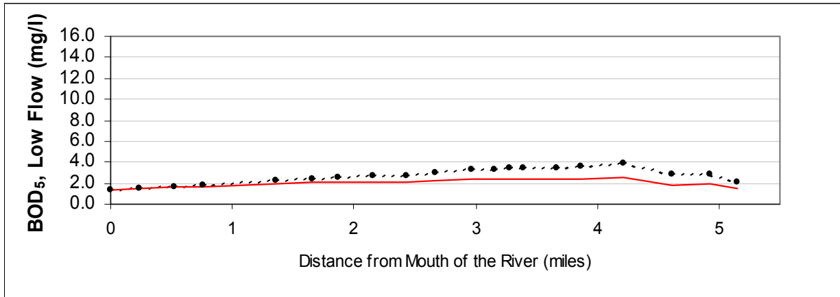
Figure A43: Dissolved Oxygen vs. River Mile for the Future Low Flow TMDL Scenario
