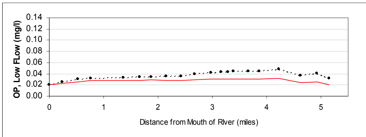
Figure A48: Organic Phosphorus vs. River Mile for the Future Low Flow TMDL Scenario
