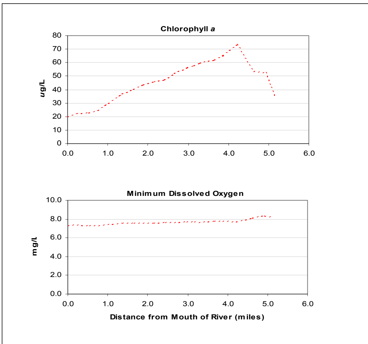
Figure 9: Model Results for the Low Flow Baseline Scenario for Chlorophyll a and Dissolved Oxygen (First Scenario)
