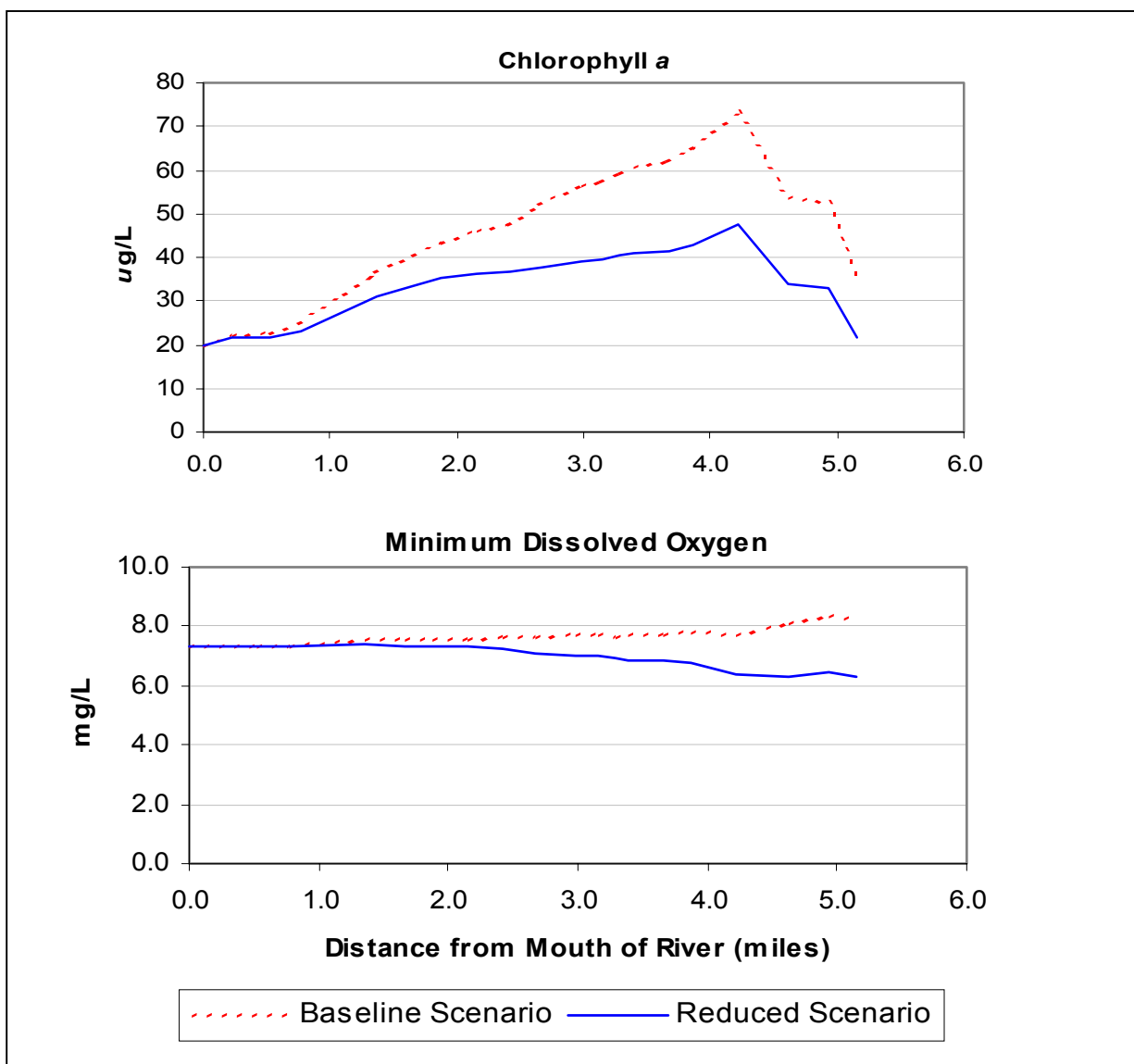
Figure 11: Model Results for the Low Flow Future Condition Scenario for Chlorophyll a and Dissolved Oxygen (Third Scenario)
