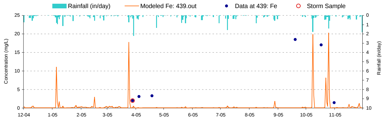
Figure E-41. Iron validation plot for Mill Run (WM-111/MIL0001)
