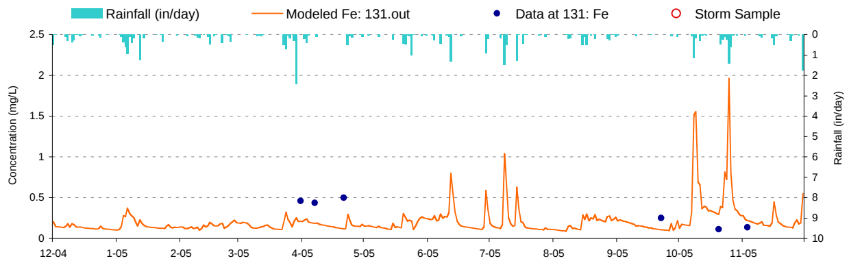
Figure E-50. Iron validation plot for North Branch Casselman River (WM-145/NBC0090)
