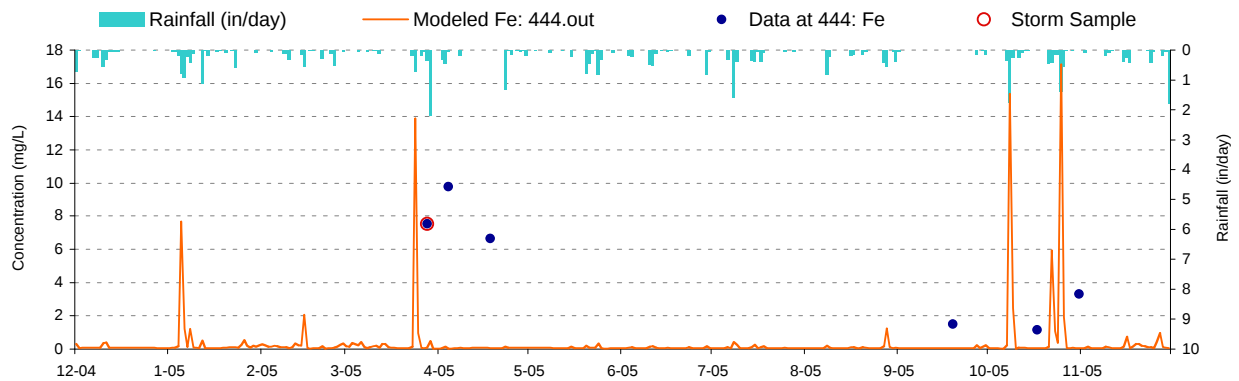
Figure E-44. Iron validation plot for Winebrenner Run (WM-120/WBN0010)
