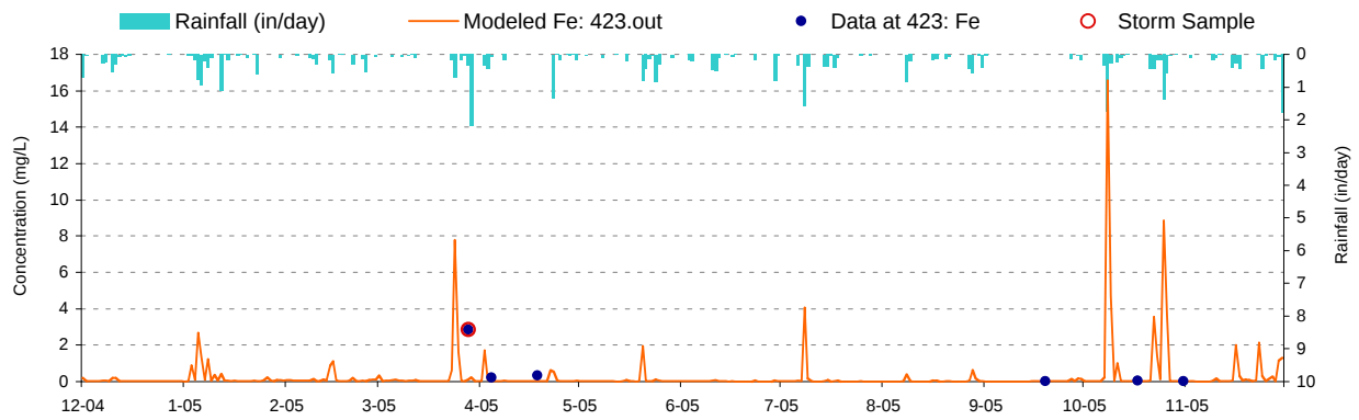
Figure E-16. Iron calibration plot for Jackson Run (WM-113/JAC0001)
