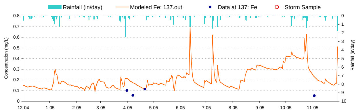
Figure E-23. Iron calibration plot for Tarkiln Run (WM-146/TAR0003)
