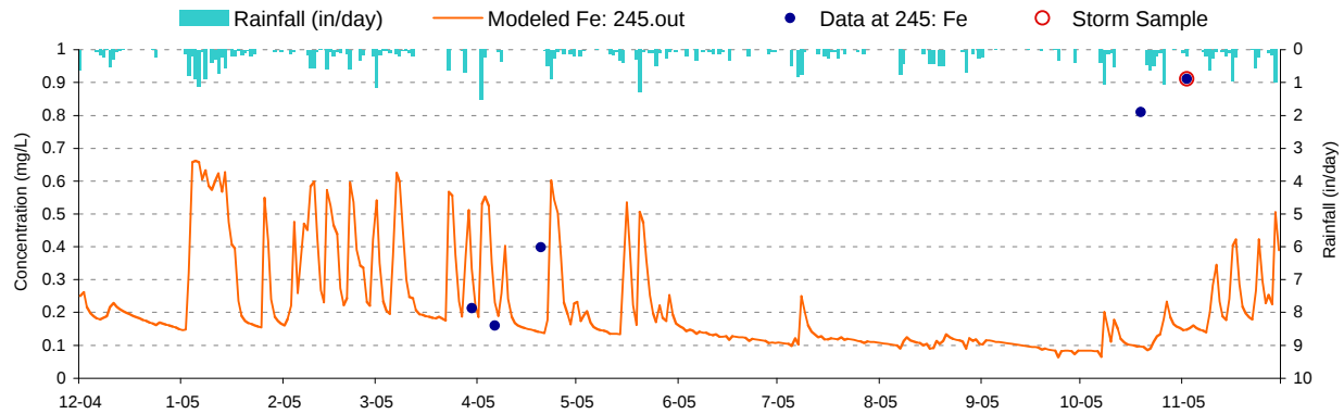
Figure E-13. Iron calibration plot for Little Savage River (WM-86/LSA0028)
