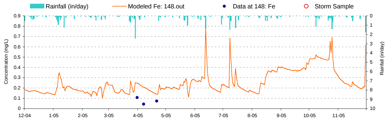
Figure E-47. Iron validation plot for Little Laurel Run (WM-137/LLR0024)
