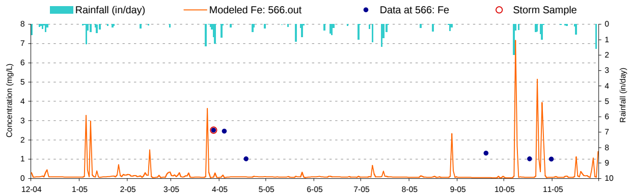
Figure E-29. Iron validation plot for UT to Jennings Run (WM-41/UJH0011)
