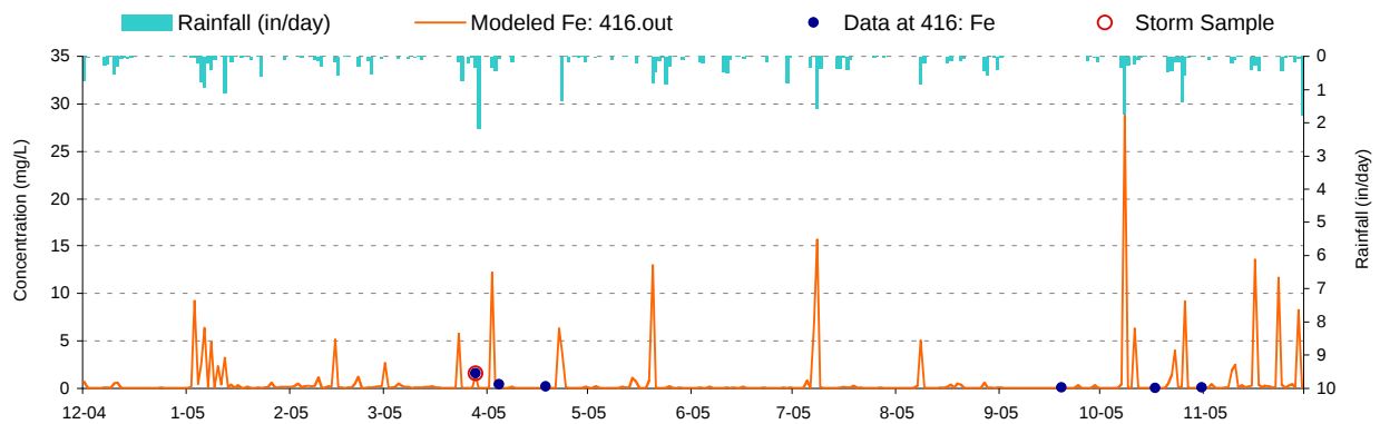
Figure E-45. Iron validation plot for UT to Moores Run (WM-122/UMD0000)
