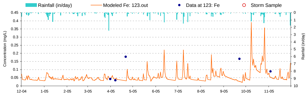
Figure E-48. Iron validation plot for Spiker Run (WM-138/SPI0018)
