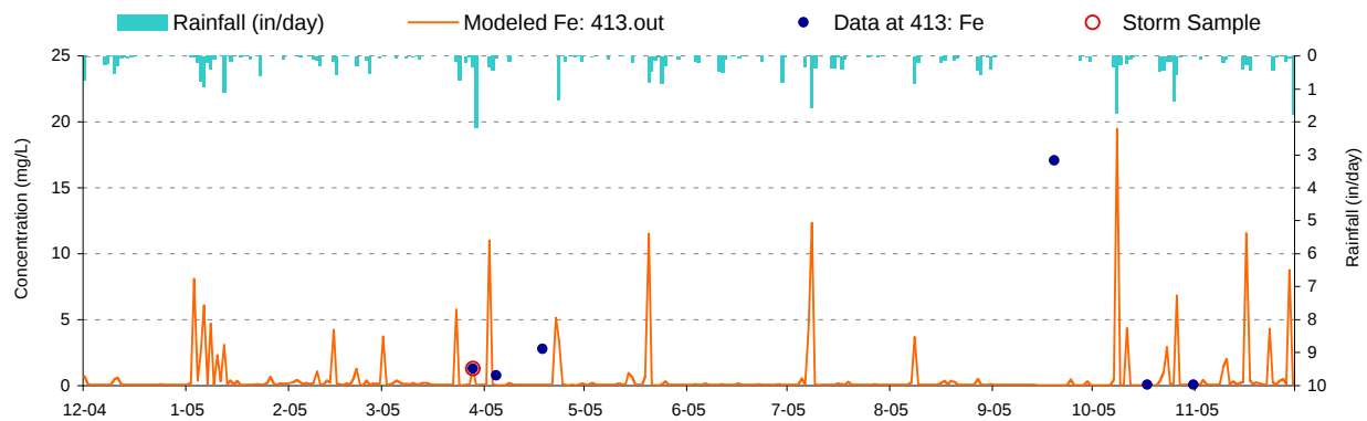
Figure E-15. Iron calibration plot for UT to Georges Creek (WM-110/UGQ0000)
