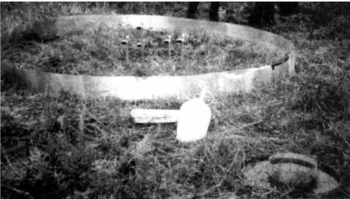
Figure 3-13. U.S. Army Corps of Engineers (USACE) Basin Test.
